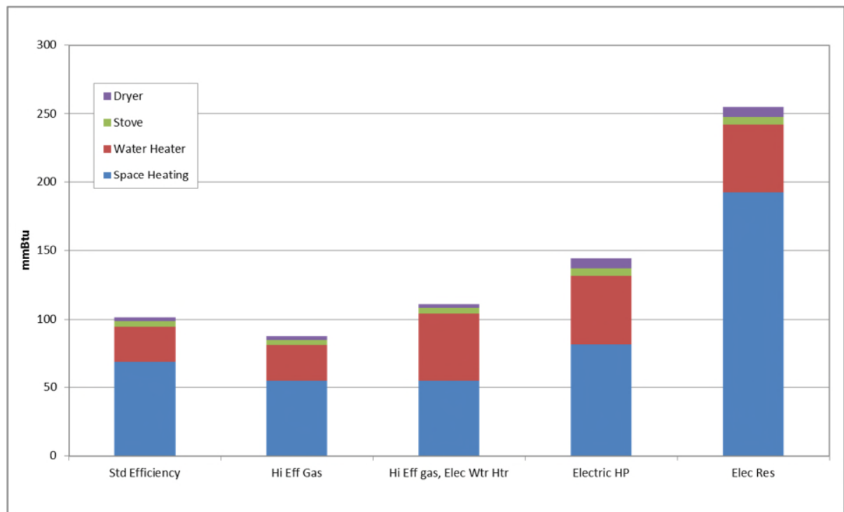
Figure 5 Energy Consumption Impacts of Fuel Switching
