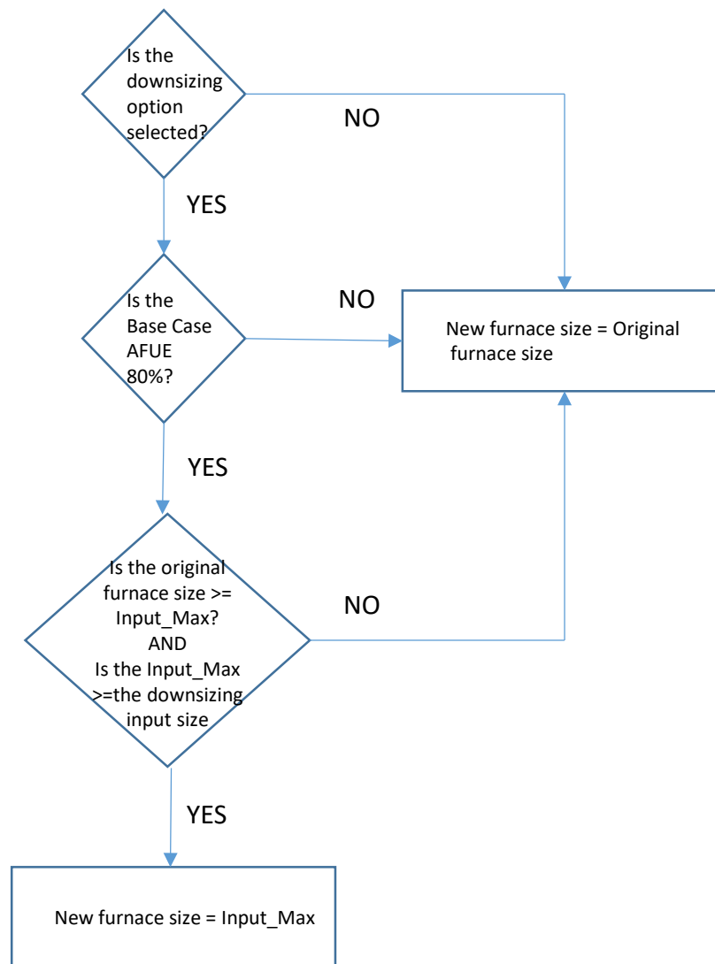
Figure 16 DOE SNO PR Furnace Down-Sizing Methodology
